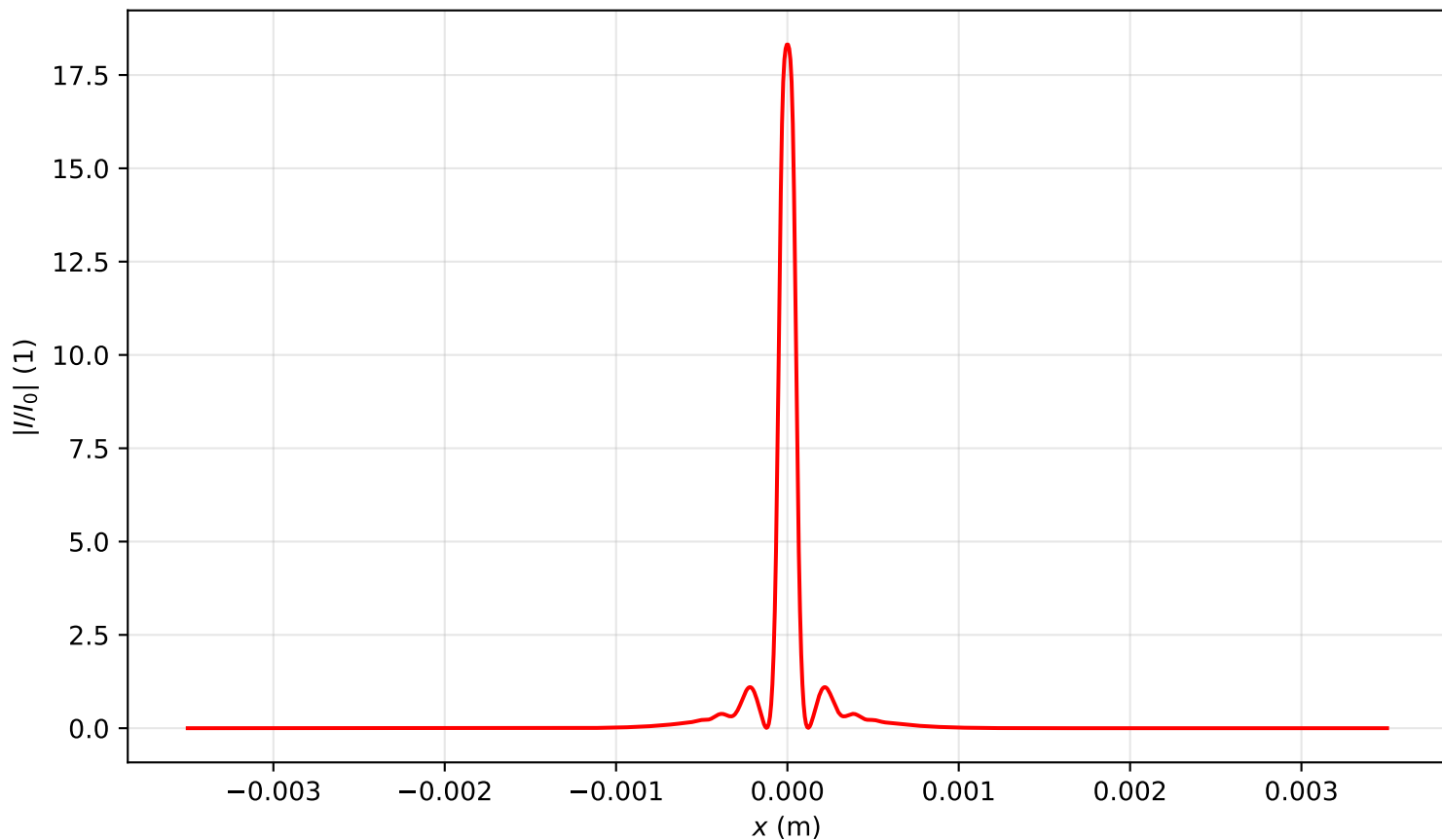
Intensity profile I(x, y = 0, z = 0.478)/I_0 , P_{in}=6.0P_{cr} , artificial time
